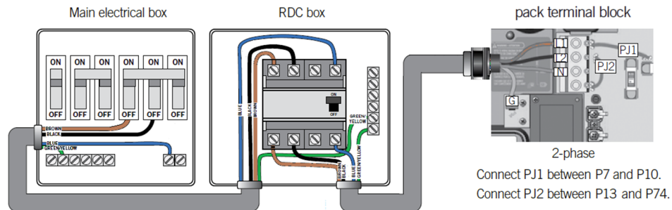
Electrical wiring: European model in.ye – in.yt
