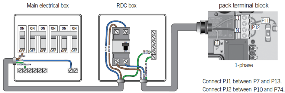
Electrical wiring: European model in.ye – in.yt
